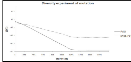
FIGURE 1. LD(t) of PSO and MXUPG of Ackley function.
