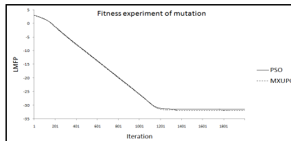
FIGURE 2. LMFPs of PSO and MXUPG of Ackley function.
